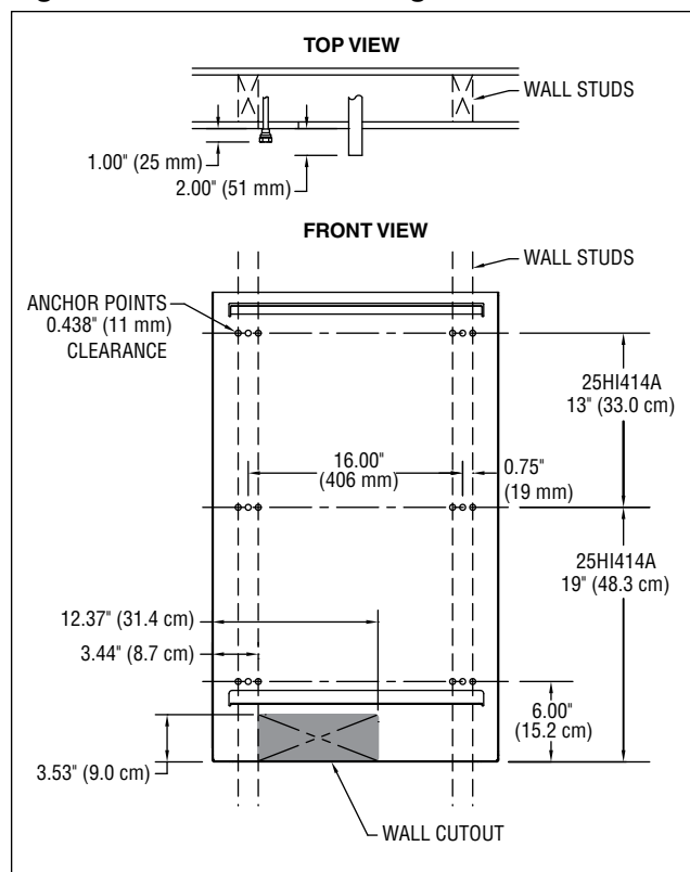
Fig. 8 – Wall bracket location guide
